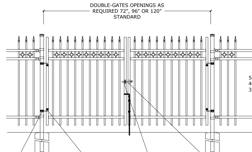
2" SQ. GRAVITY-CATCH (LOCKABLE)
