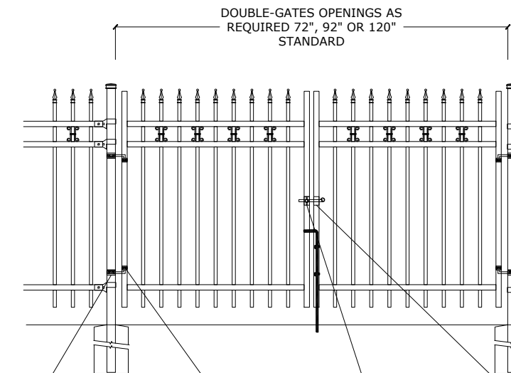
2" SQ POST-COLLAR C/W 1/2 DIA X 4" HINGE BOLT
