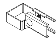
MULTI-FUNCTIONAL BRACKET
