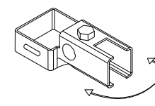
SWIVEL BRACKET
