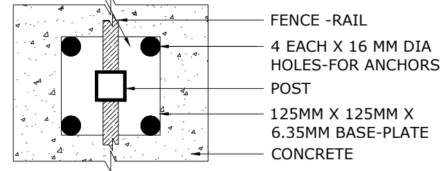
BASE-PLATE (OPTIONAL)
