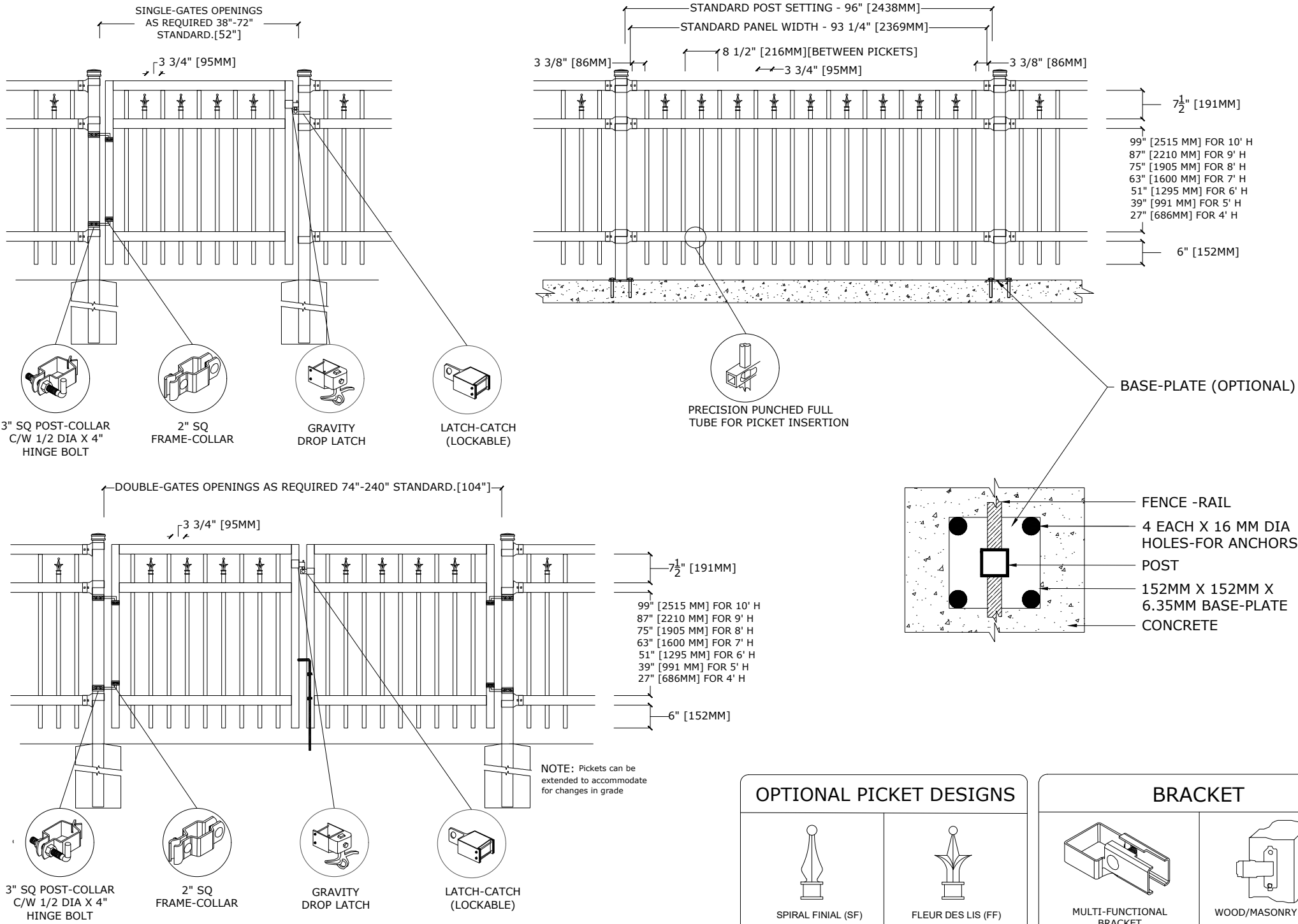
MULTI-FUNCTIONAL BRACKET
