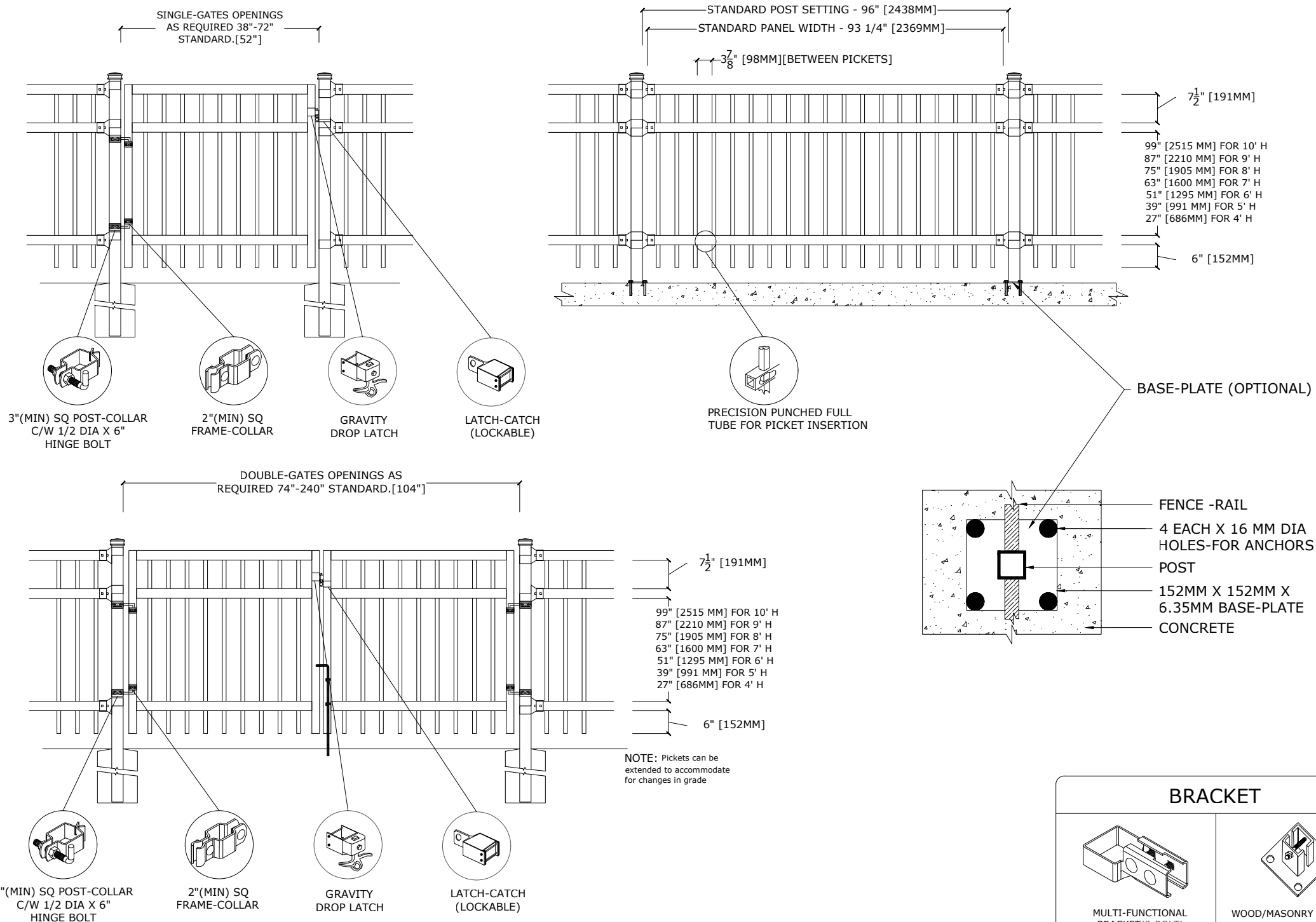
MULTI-FUNCTIONAL BRACKET(2-BOLT)
