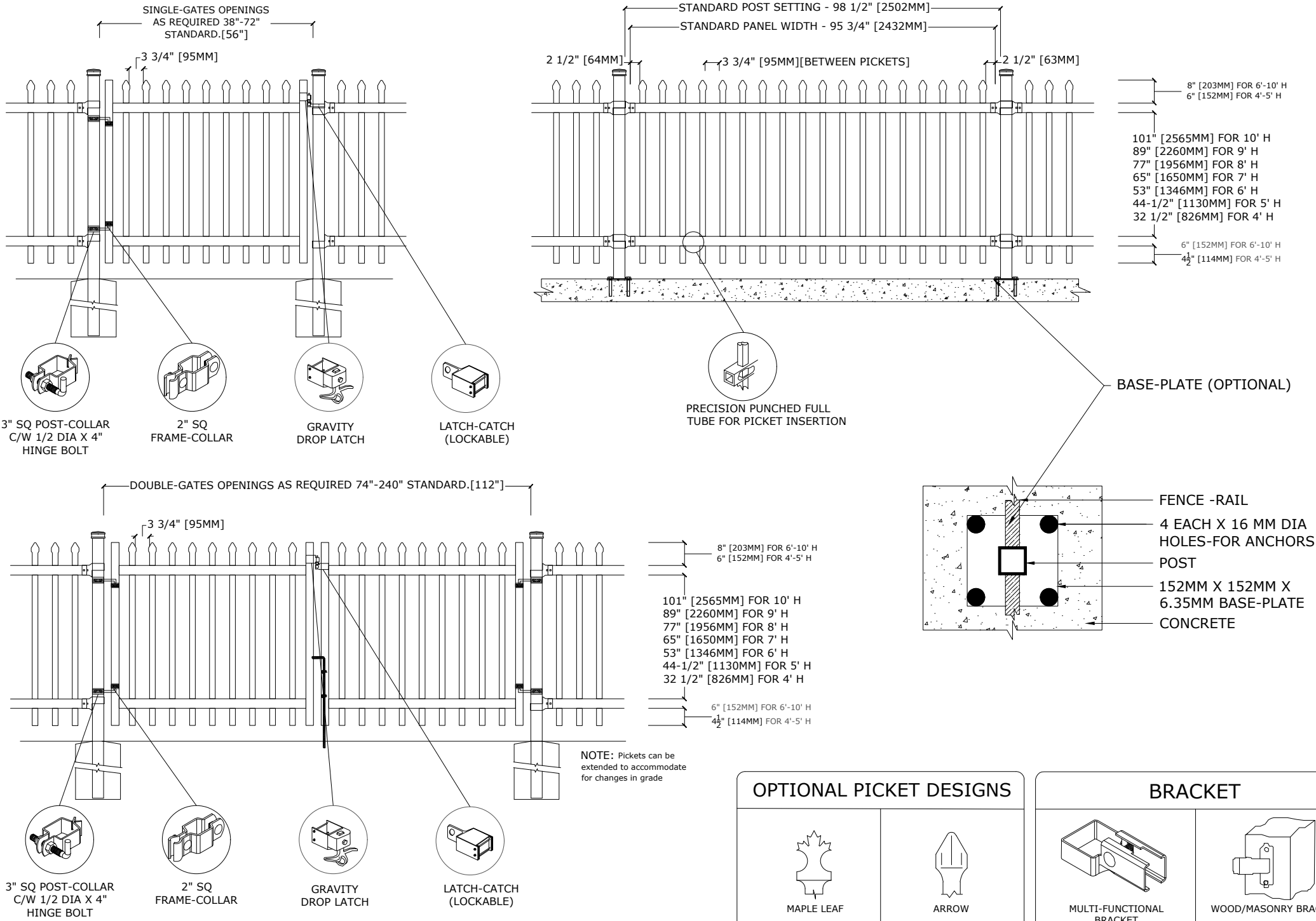
MULTI-FUNCTIONAL BRACKET
