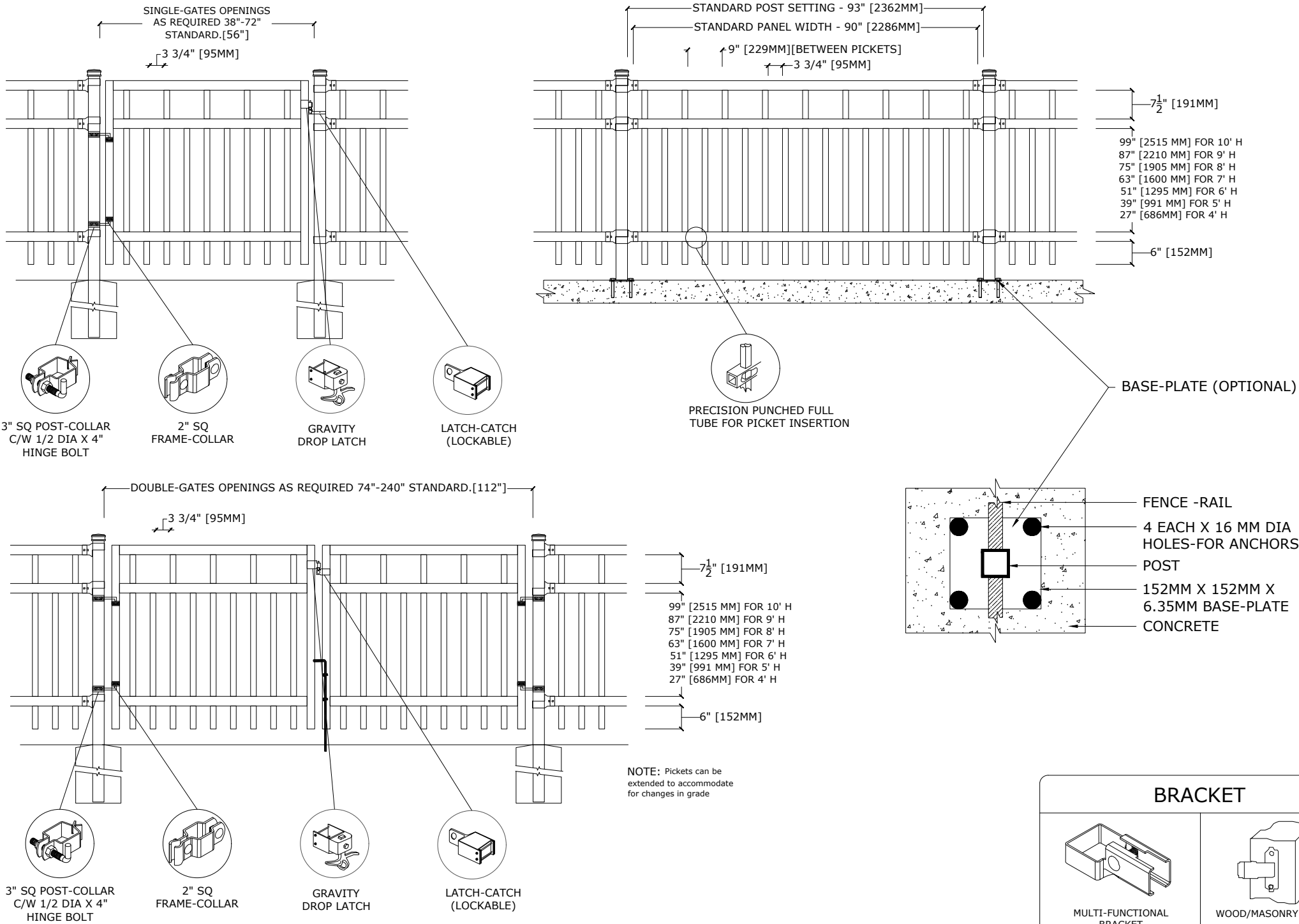
MULTI-FUNCTIONAL BRACKET
