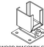
WOOD/MASONRY SWIVEL BRACKET
